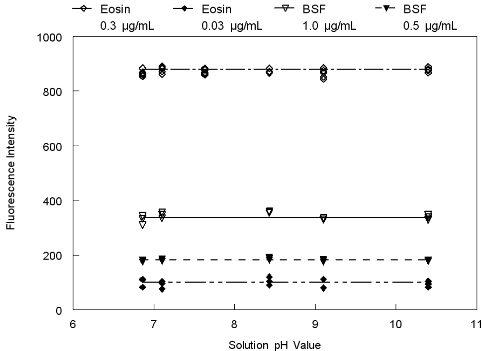
FIG. 3—Effect of final solution pH conditions on fluorescent intensities of solutions containing 0.03 and 0.3 \mu\text{g/mL} Eosin and 0.5 and 1.0 \mu\text{g/mL} BSF, respectively.
